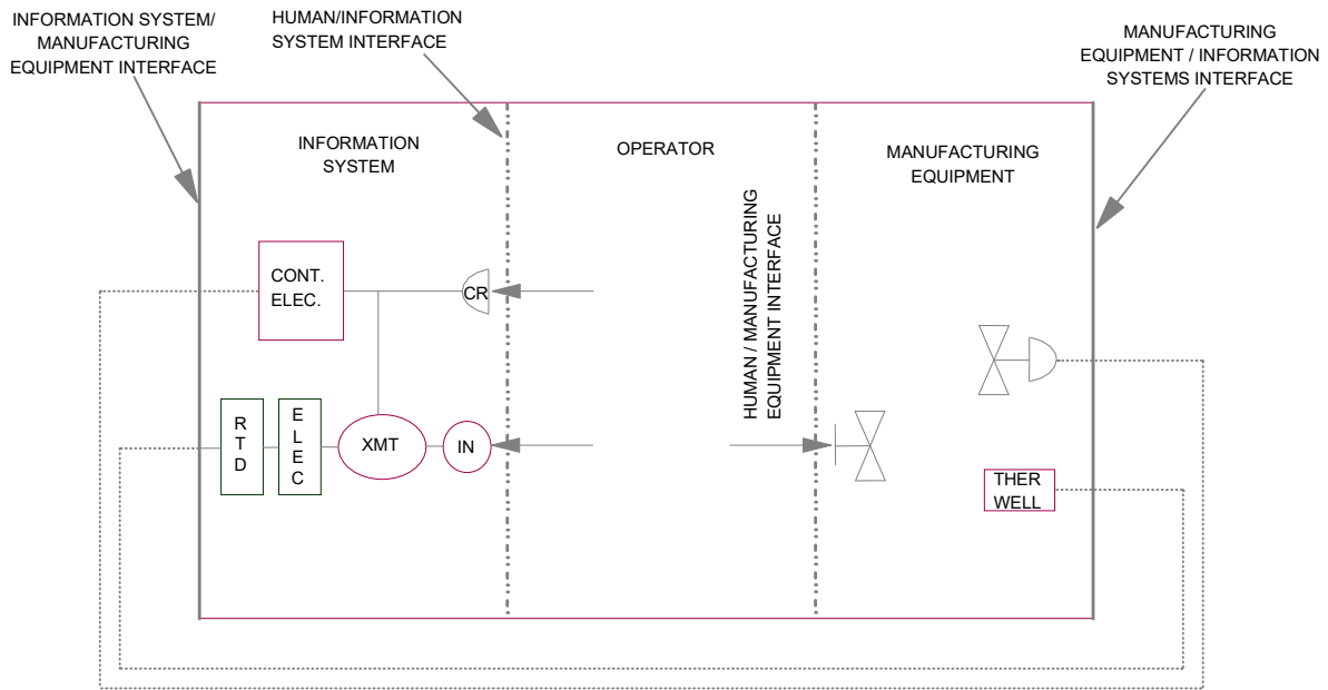
FIGURE 9-4 INTERFACES IN THE OVERALL ENTERPRISE INTEGRATION SYSTEM
