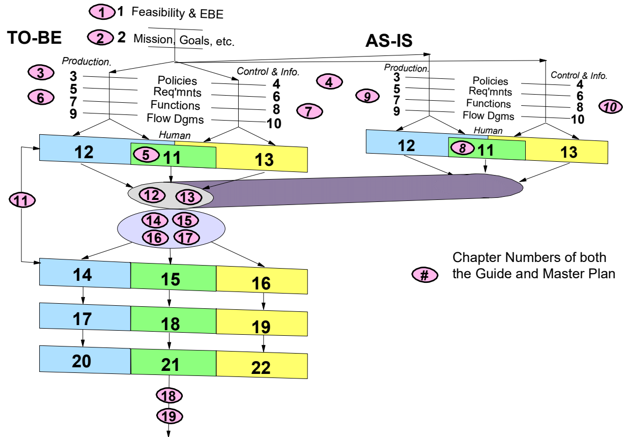
FIGURE 9-2 THE WORK OF CHAPTER 9 DEFINES REQUIREMENTS OF THE AS-IS MANUFACTURING EQUIPMENT ARCHITECTURE AS SHOWN BY PERA
