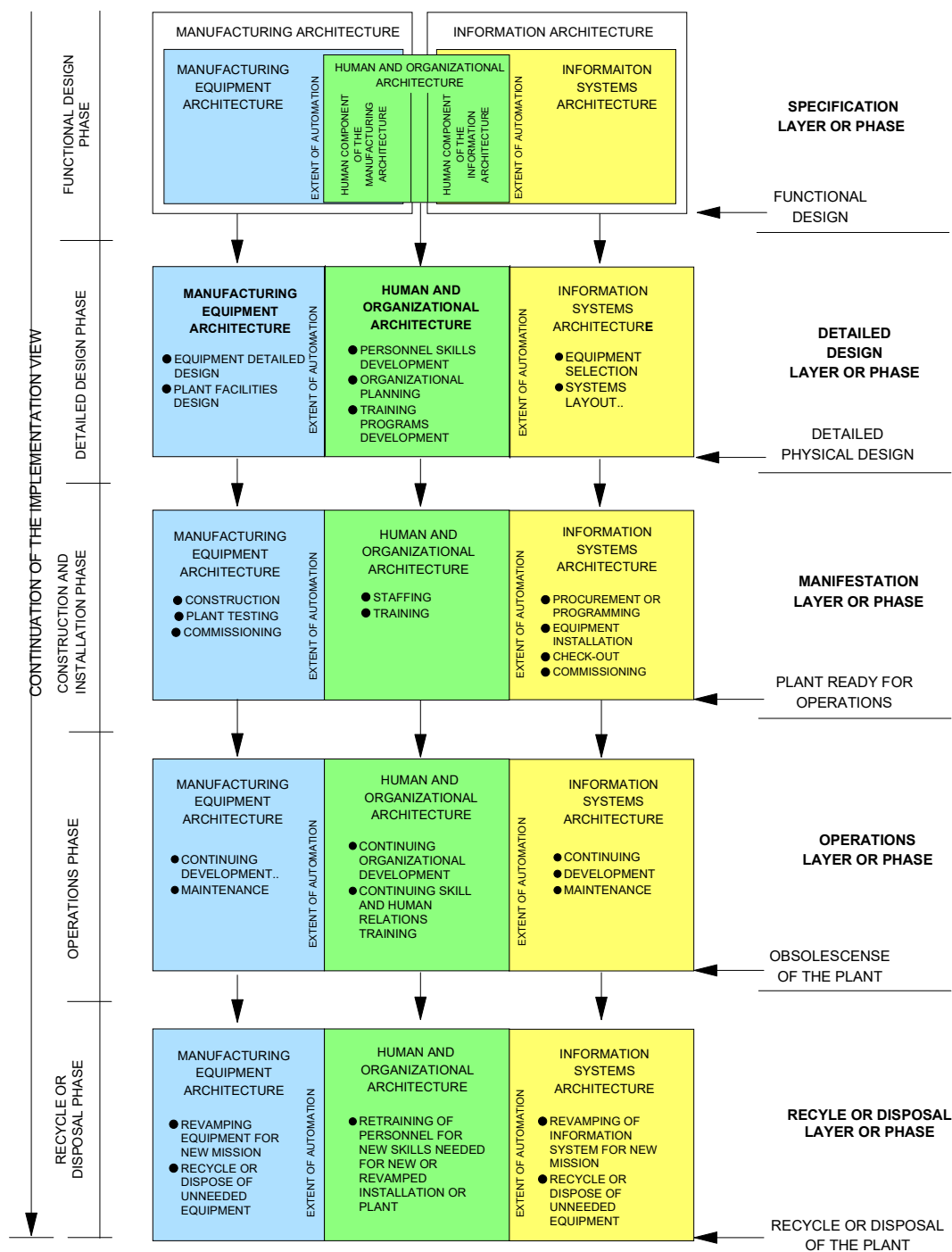
FIGURE 6B ENTERPRISE PHASES RELATED TO PURDUE ARCHITECTURE LAYERS OR PHASES
